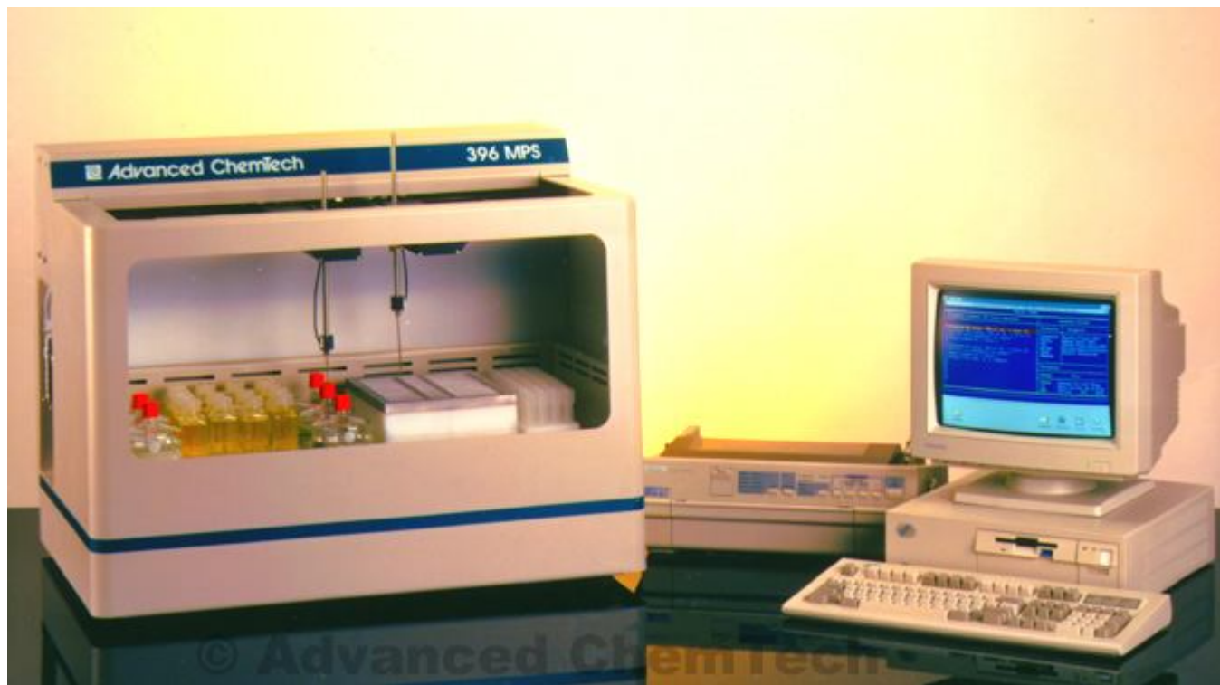
The Advanced ChemTech (ACT) model 396MPS automatic peptide synthesizer.
